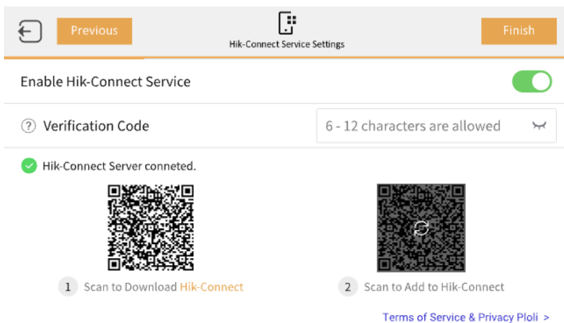
Figure 2-11 Cloud Service-LAN
