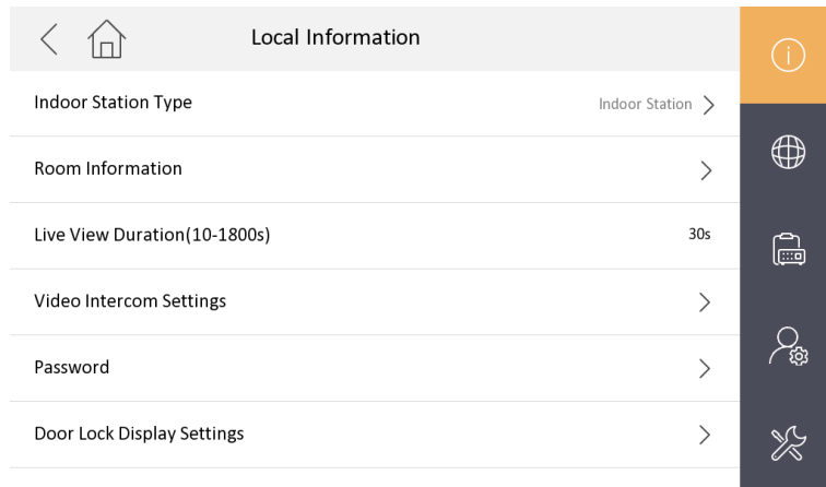
Figure 2-27 Local Information
