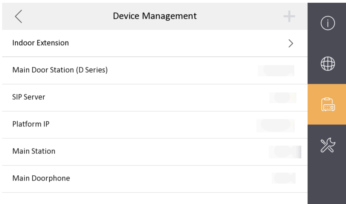
Figure 2-16 Device Information
