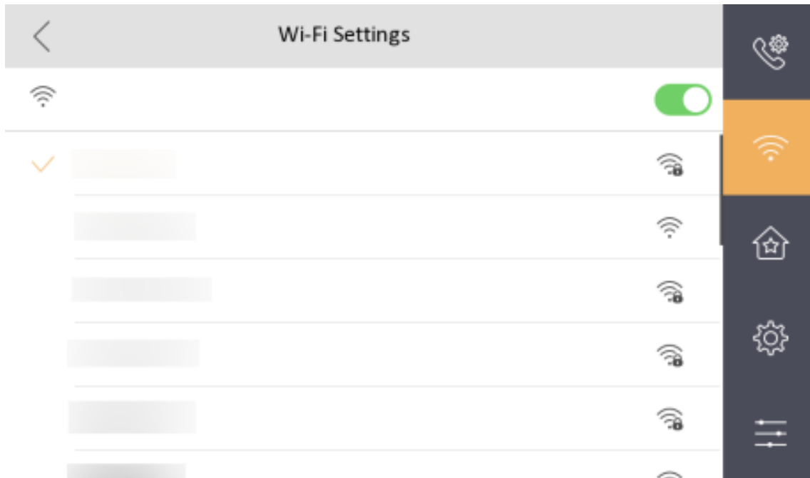
Figure 2-14 Wi-Fi Settings
