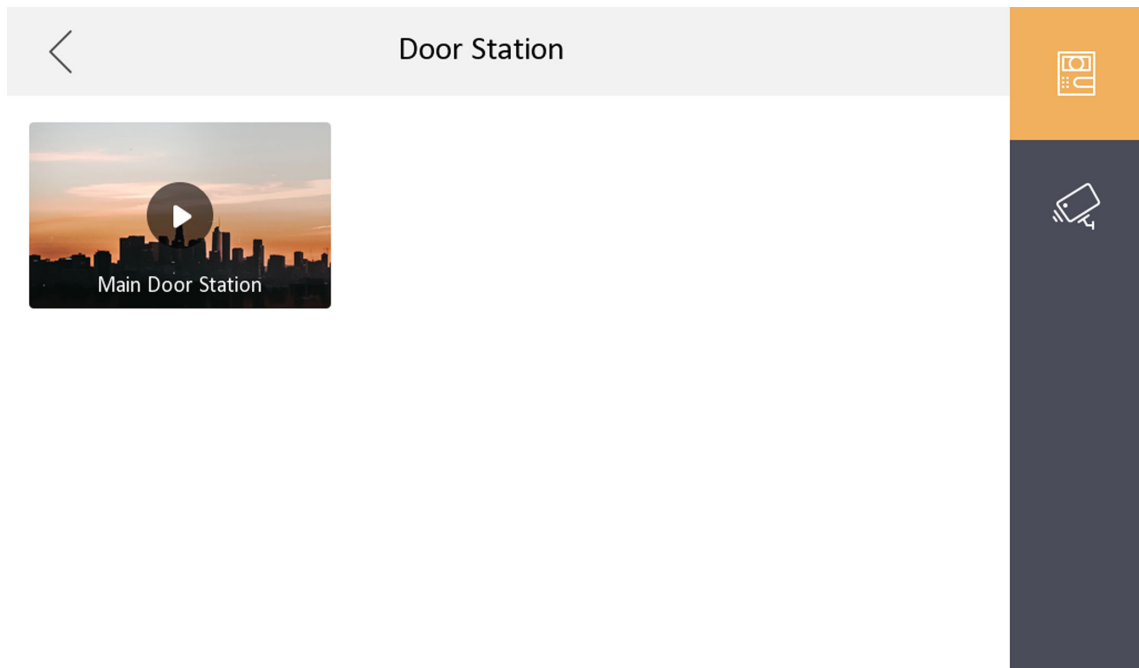
Figure 4-8 Live View
