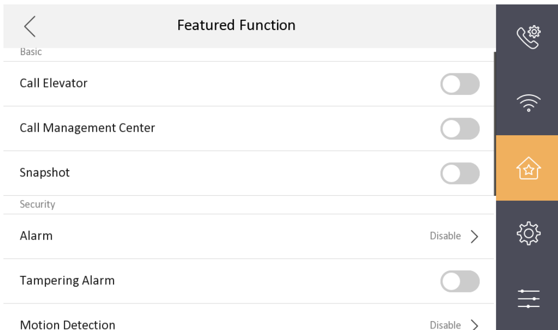
Figure 2-31 Featured Function
