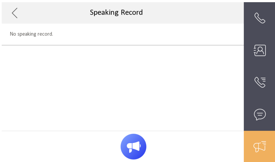
Figure 4-11 Speaking Record
