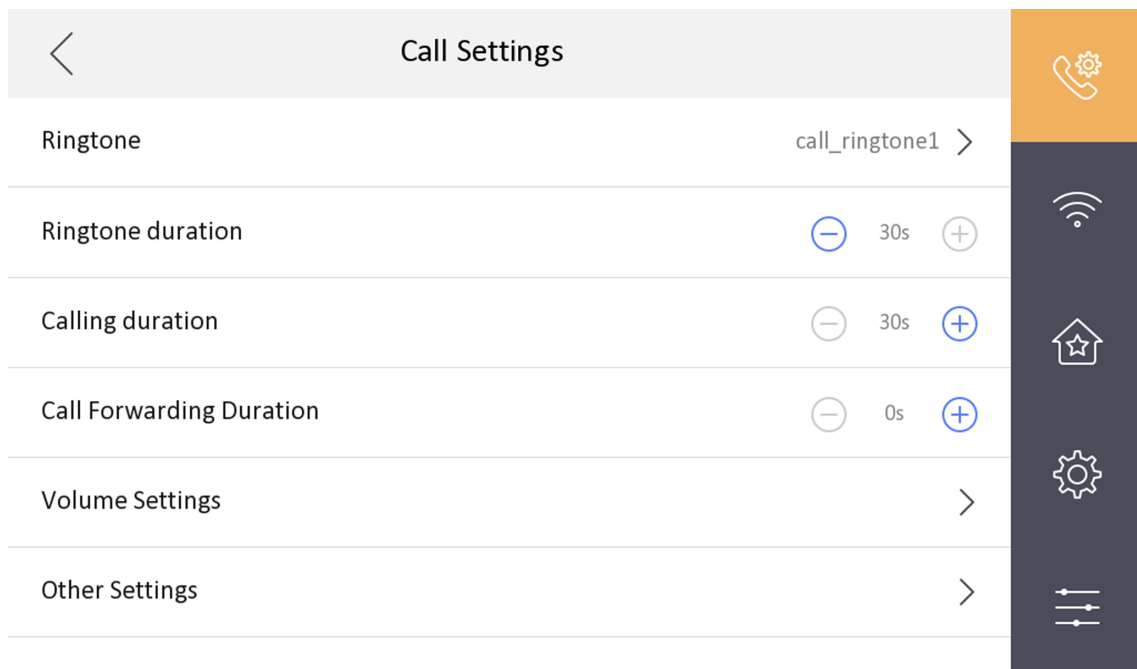
Figure 2-34 Call Settings
