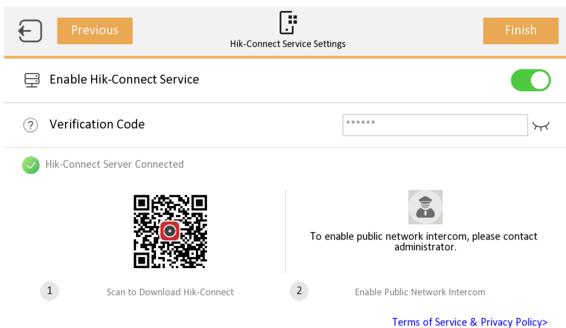
Figure 2-12 Cloud Service-WAN
