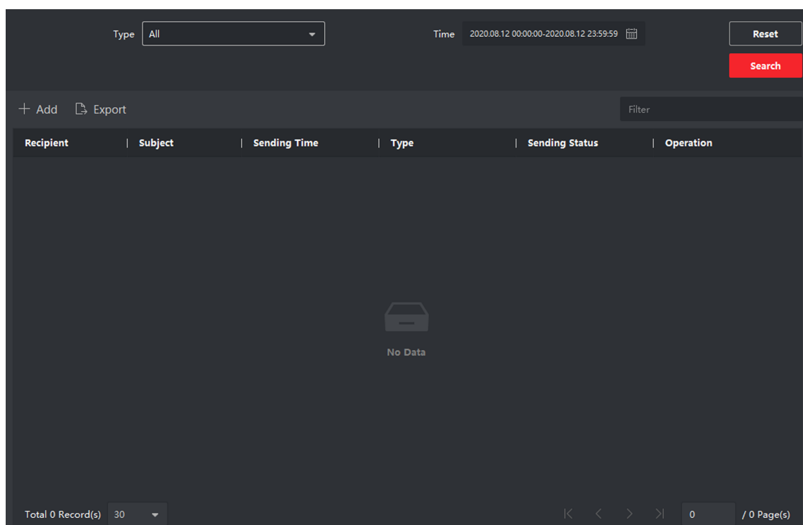
Figure 5-22 Release Notice
