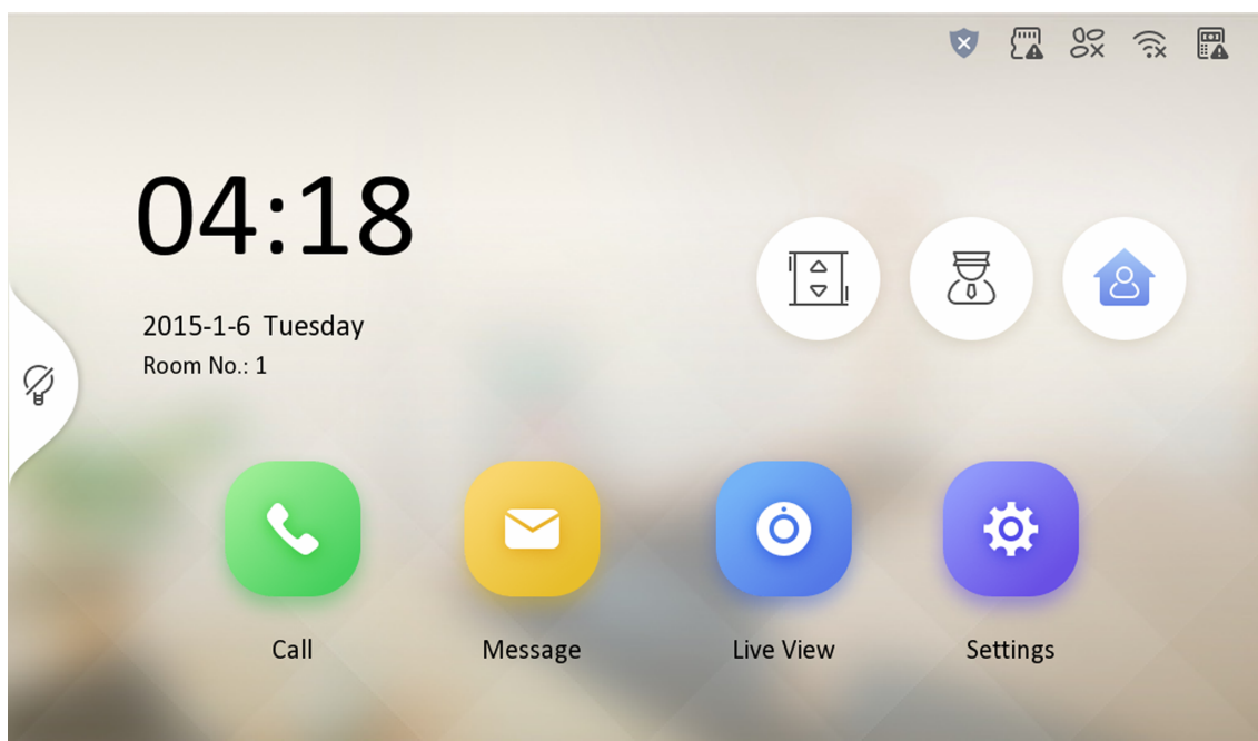
Figure 2-35 Main Page
