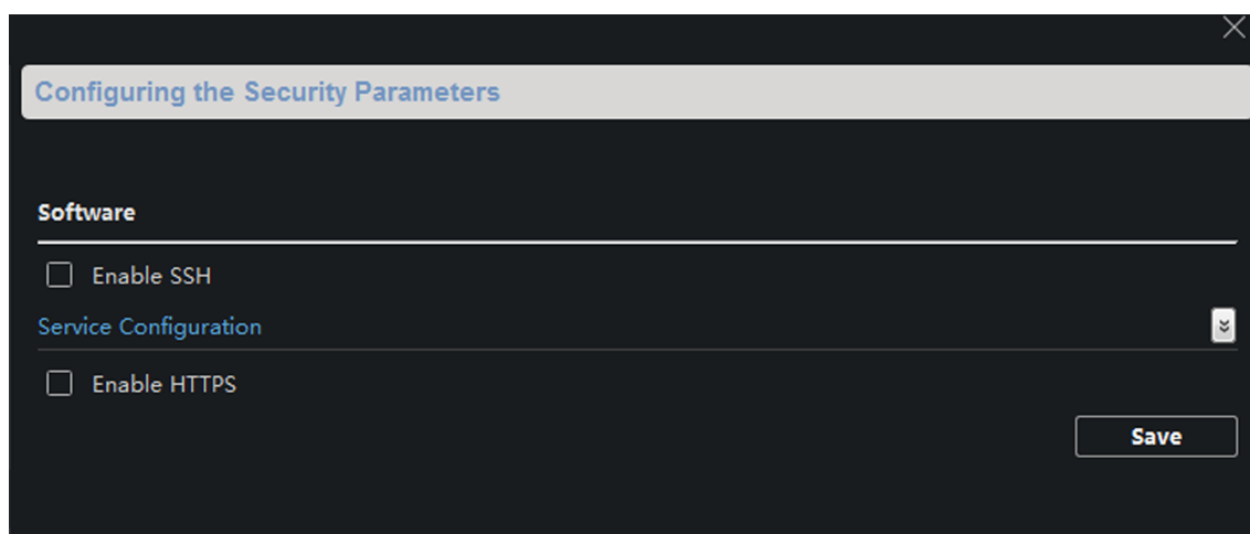
Figure 5-8 Security
