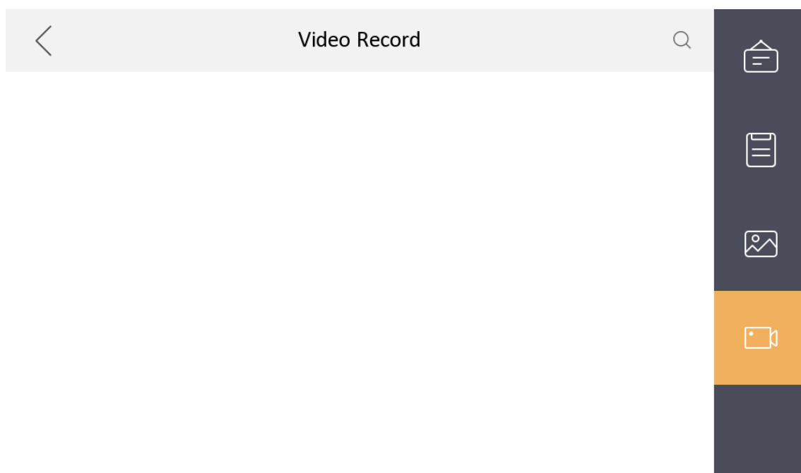
Figure 4-13 Video Record
