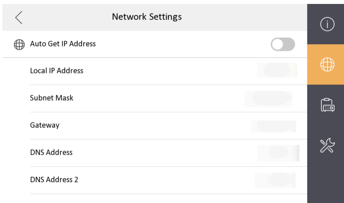
Figure 2-13 Network Information
