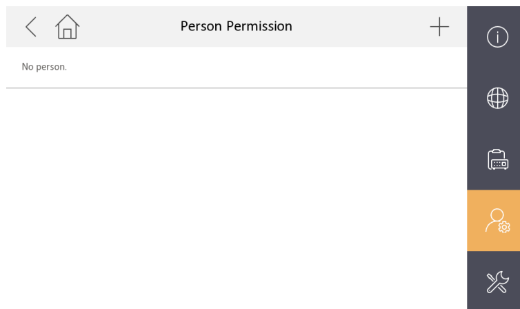
Figure 2-37 Person Permssion
