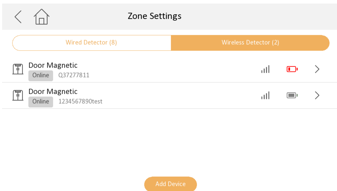
Figure 2-20 Zone Settings
