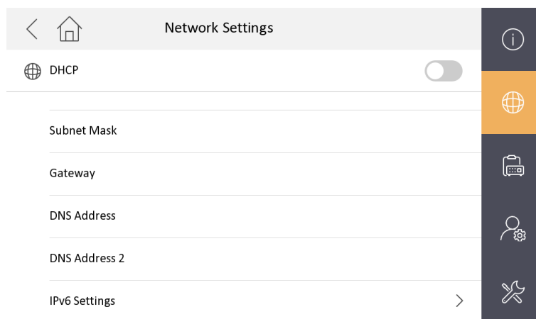
Figure 2-17 Network Settings-IPv6
