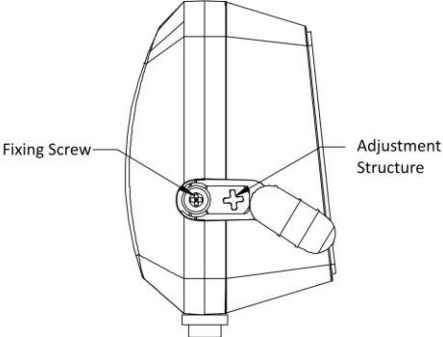
Figure 2-4 Adjust the Angle
