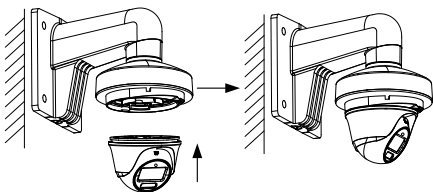
Figure 2-25 Finish Installation
