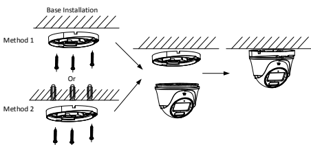
Figure 2-18 Install the Camera to Ceiling
