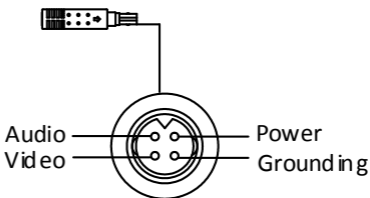
Figure 1-2 Interfaces of 4-Pin Din Connector
