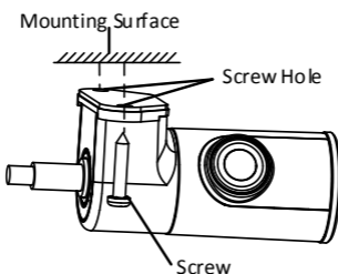
Figure 2-4 Fix the Camera
