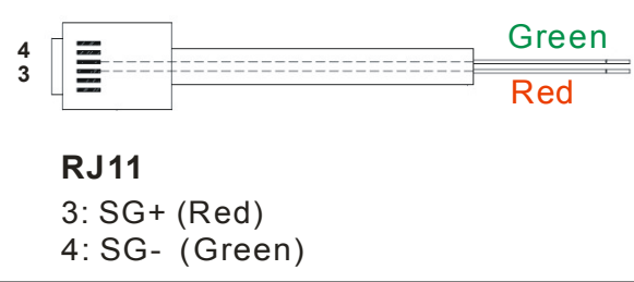
Figure 5 IFD6500 accessory RJ11 ↔ RS-485
